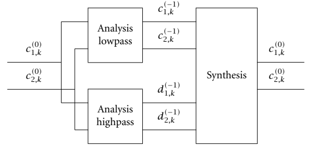
FIGURE 1: Analysis-synthesis scheme.
