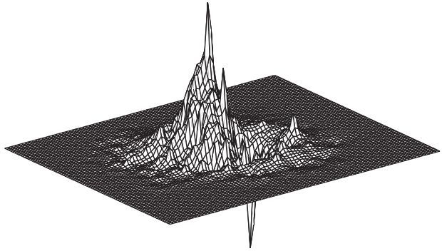
FIGURE 7: Scaling function 2.
