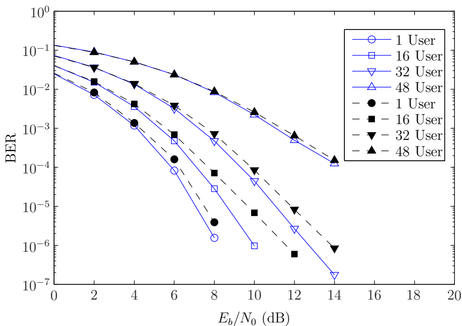
Figure 6 BER comparison for OFDM-CDMA system with 4Tx, 4Rx with our proposed scheme (solid) and DOC-STFS-CDMA [9](dotted) in a slow fading frequency-selective environment.
