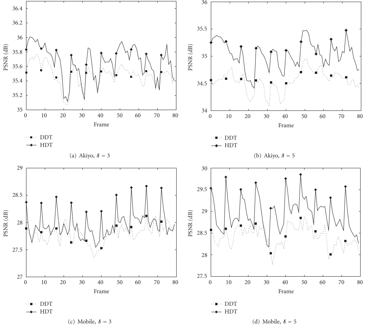
FIGURE 8: PSNR obtained by downscaling the Akiyo and Mobile video sequences, considering Q = 4 and \text{GOP} = 8 frames.
