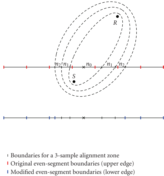
FIGURE 2: Unfolded 2D view of a source, receiver, and segmented edge. The upper edge is marked with the boundaries for a 3-sample alignment zone (samples n_0 , n_1 , and n_2 ) in black and the original even-segment boundaries in red. The lower edge ( S and R not shown) is marked with the modified segment boundaries for the hybrid subdivision scheme in blue: even segments overlapping the alignment zone have been truncated at the edges of the zone, and those completely within the alignment zone have been discarded. The apex point is marked with an “x.”
