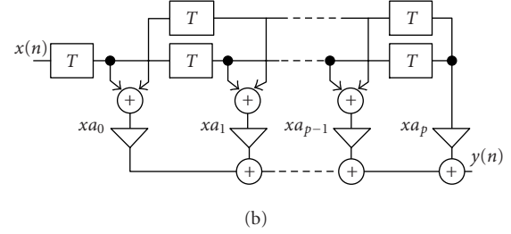
FIGURE 9: Realization of FIR filter: (a) simple direct structure and (b) direct structure for a linear phase filter.
