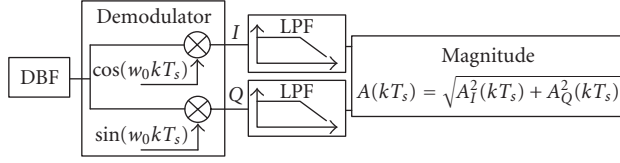
FIGURE 8: Quadrature sampling technique for bandpass signals.
