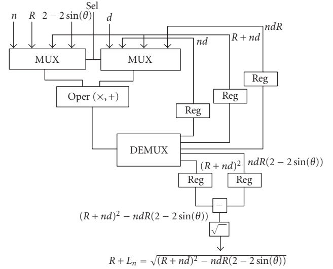
FIGURE 7: Block diagram of the delay time distance calculation.
