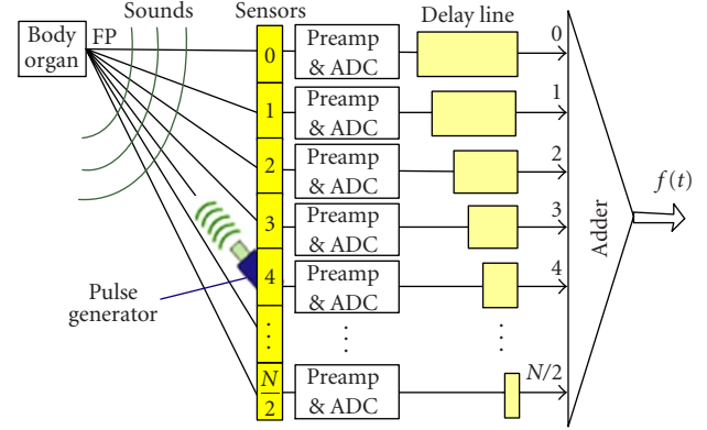
FIGURE 3: Simplified schematic of the pipelined digital beamforming.
