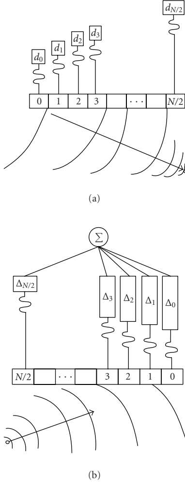
FIGURE 2: Beamforming: (a) resulting focal point, and (b) delay generation.
