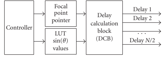
FIGURE 5: Proposed delay calculation architecture.
