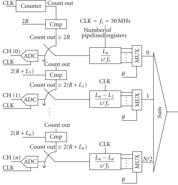
FIGURE 6: Block diagram of the pipelined sampled-delay.
