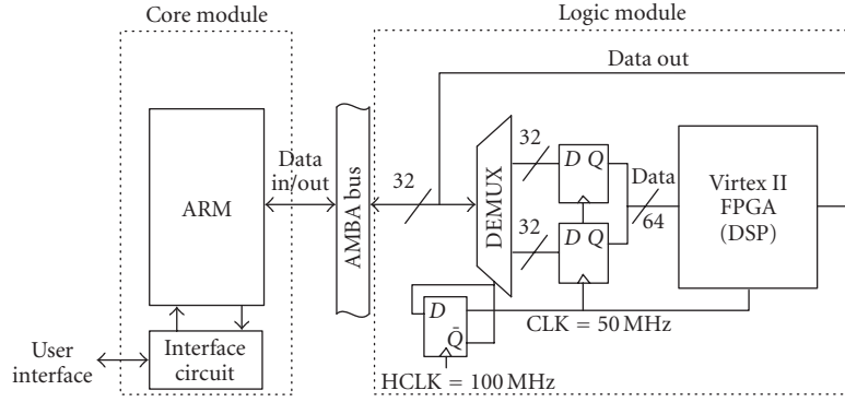
FIGURE 10: Block diagram of the ARM platform used for DSP core implementation.
