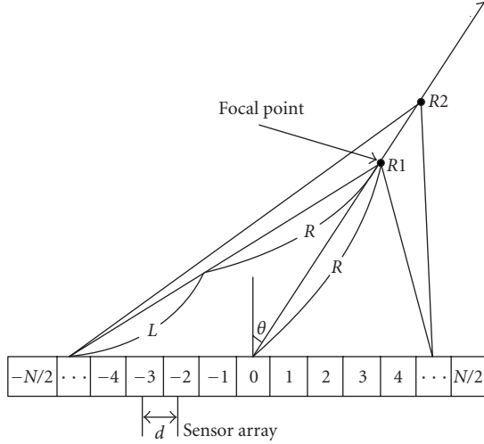
FIGURE 4: Dynamic focusing and steering delay.
