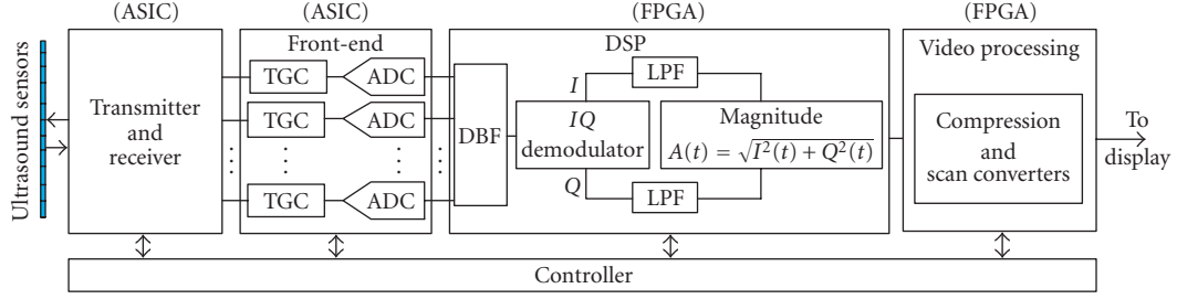
FIGURE 1: Perception SoC of the B-mode processing of the ultrasonic imaging system.
