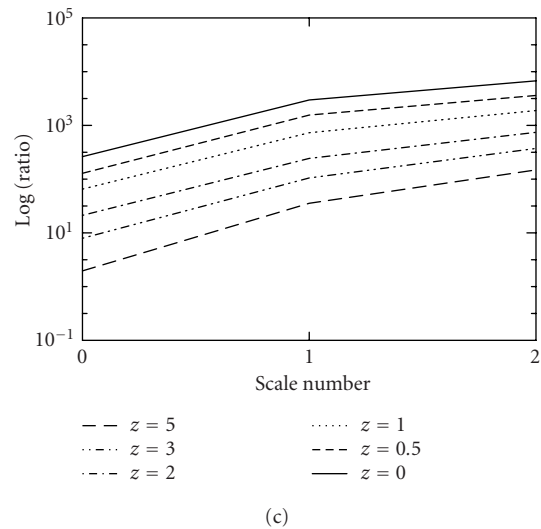
FIGURE 15: (a) Wavelet spectrum, (b) beamlet spectrum, and (c) ridgelet spectrum at different redshifts.
