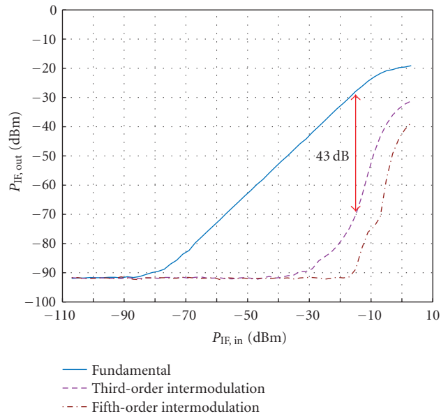
FIGURE 7: Measured intermodulation for concatenated analog IF-to-RF up- and RF-to-IF down-converter modules.
