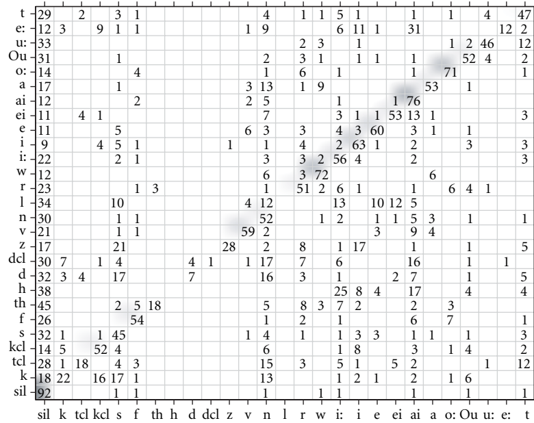
FIGURE 11: Confusion matrix of the phoneme identification from the video stream, showing percentage of each phoneme on the y-axis identified as phonemes on the x-axis.
