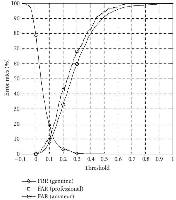
FIGURE 9: Dolfing's data set. Graphs for the FRR and the FAR when d = 512 , \Theta = 128 , N = 64 , and \ell = 1 .
