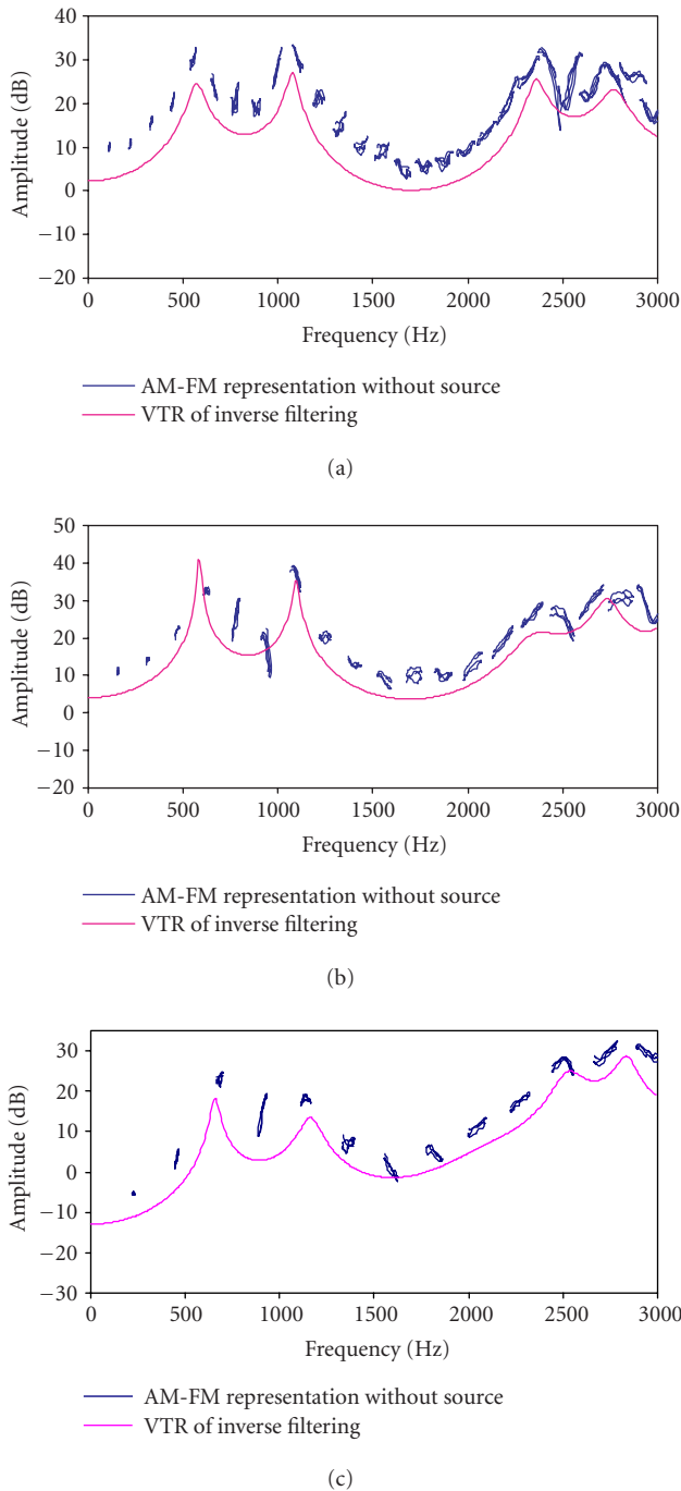
FIGURE 22: AM-FM representation removing the source and VTR given by inverse filtering. (a) F_0 = 110 Hz, vowel "a," (b) F_0 = 156 Hz, vowel "a," (c) F_0 = 227 Hz, vowel "a."
