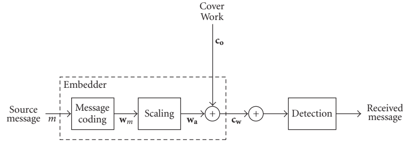
FIGURE 1: Watermarking using blind embedding.
