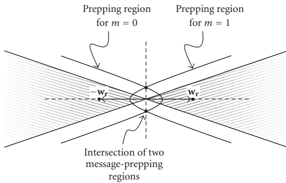
FIGURE 8: Preprocessing for a one-bit, normalized-correlation watermarking system. The one-bit detector defines two conical detection regions: one centered around w_r , for m = 1 , and one around -w_r , for m = 0 . For each detection region, there is a message-prepping region of content in which a blind embedder can embed the corresponding message. The overall prepping region is the intersection of these two message-prepping regions, which comprise two points in this two-dimensional figure.
