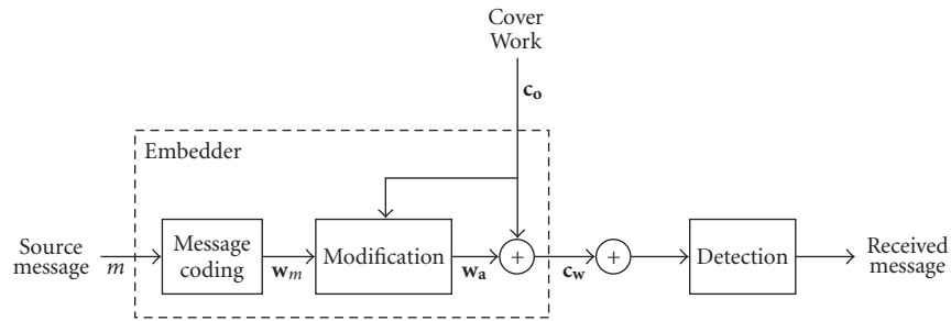
FIGURE 2: Watermarking using informed embedding.
