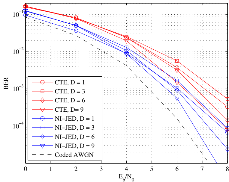
Figure 14 NI-JED and CTE performance for interleave depths D = 1, D = k, D = 2k and D = 3k , and CIR length L = 2 . Red circle: CTE, D = 1 ; Red square: CTE, D = 3 ; Red diamond: CTE, D = 6 ; Red triangle: CTE, D = 9 ; Blue circle: NI-JED, D = 1 ; Blue square: NI-JED, D = 3 ; Blue diamond: NI-JED, D = 6 ; Blue triangle: NI-JED, D = 9 ; Black dashed: Coded AWGN.
