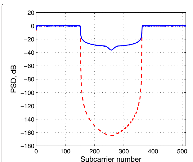
Figure 1 Power spectral densities of OFDM and OQAM signals.
