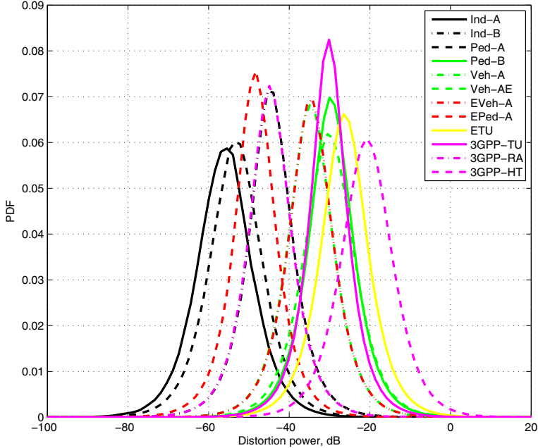
Figure 8 PDFs of FBMC distortion power for different channel models.
